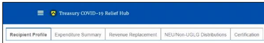
Figure 2 – Navigation Bar
