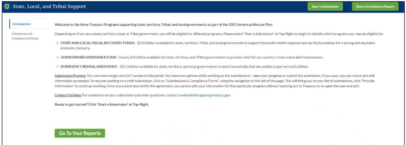
Figure 1 – Landing Page
