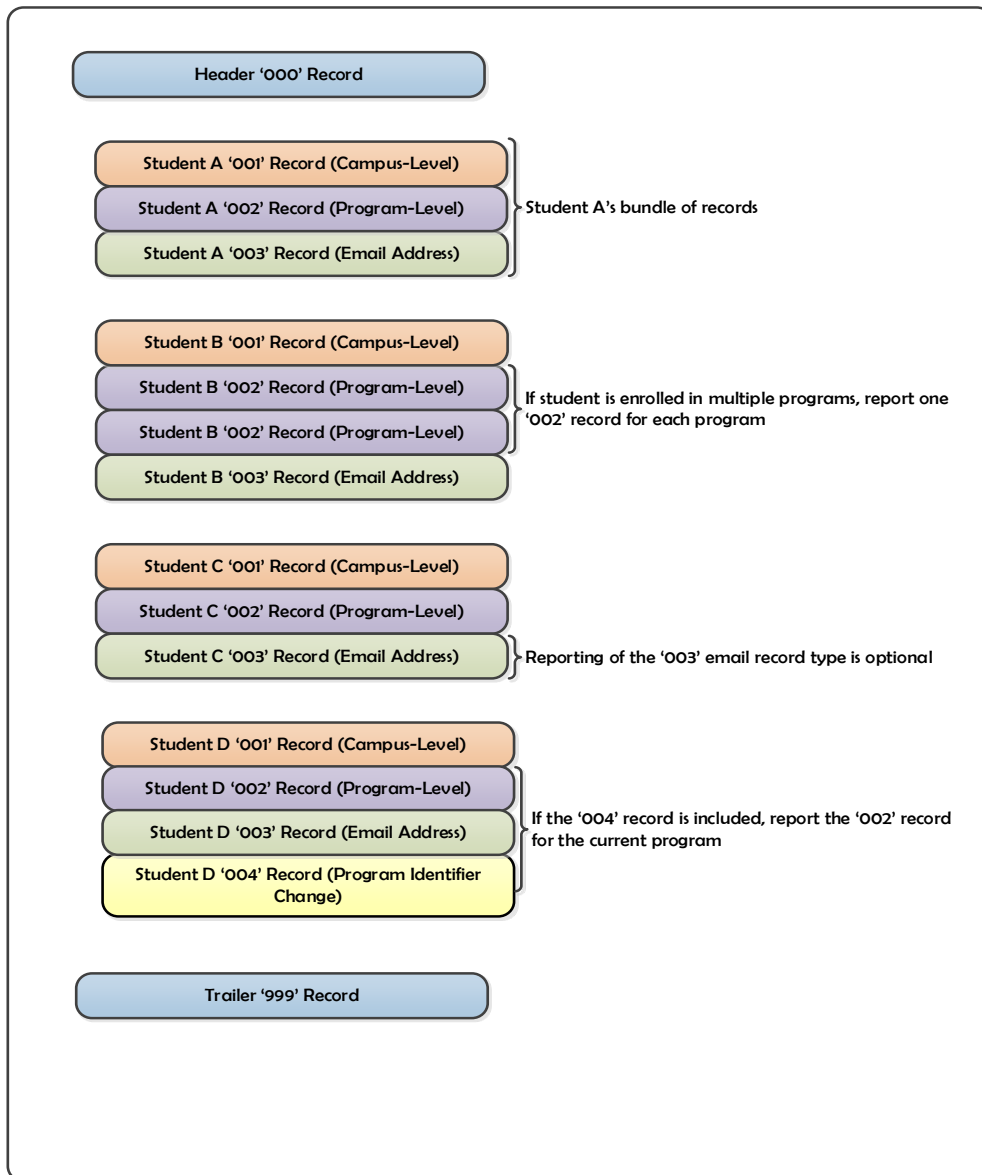
Figure 6-1: Bundle Format Example
