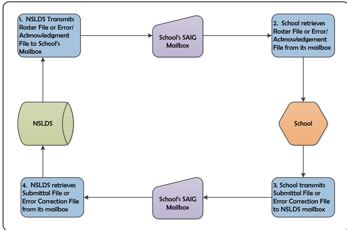
Figure 7-64: Enrollment Reporting Batch Process Flow
