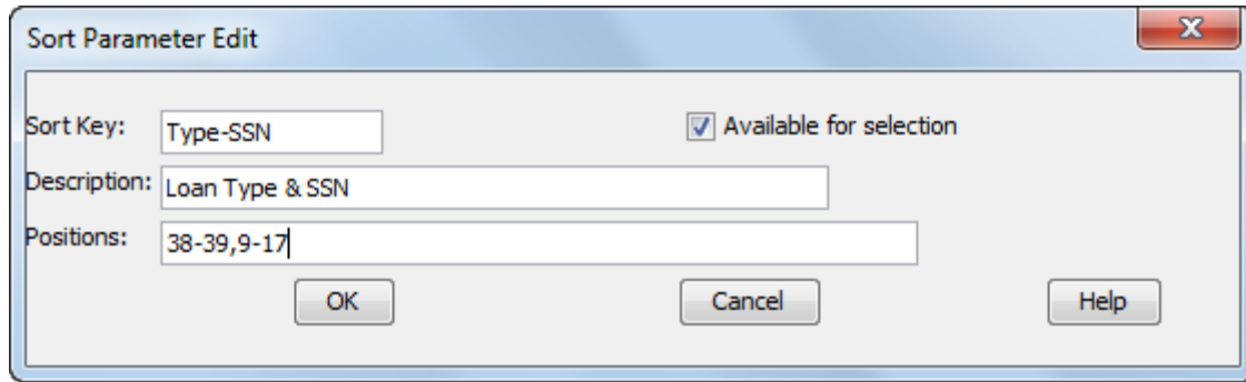
Figure 10-36: Sort Parameter Edit Dialog Box
