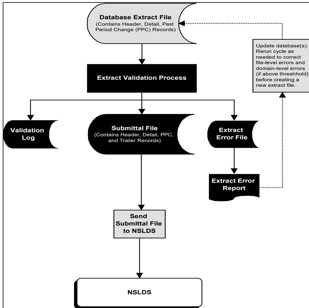
Figure 7-1: Extract Validation Process
