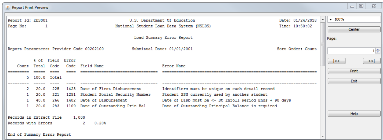
Figure 12-2: Summary Load Process Error Report
