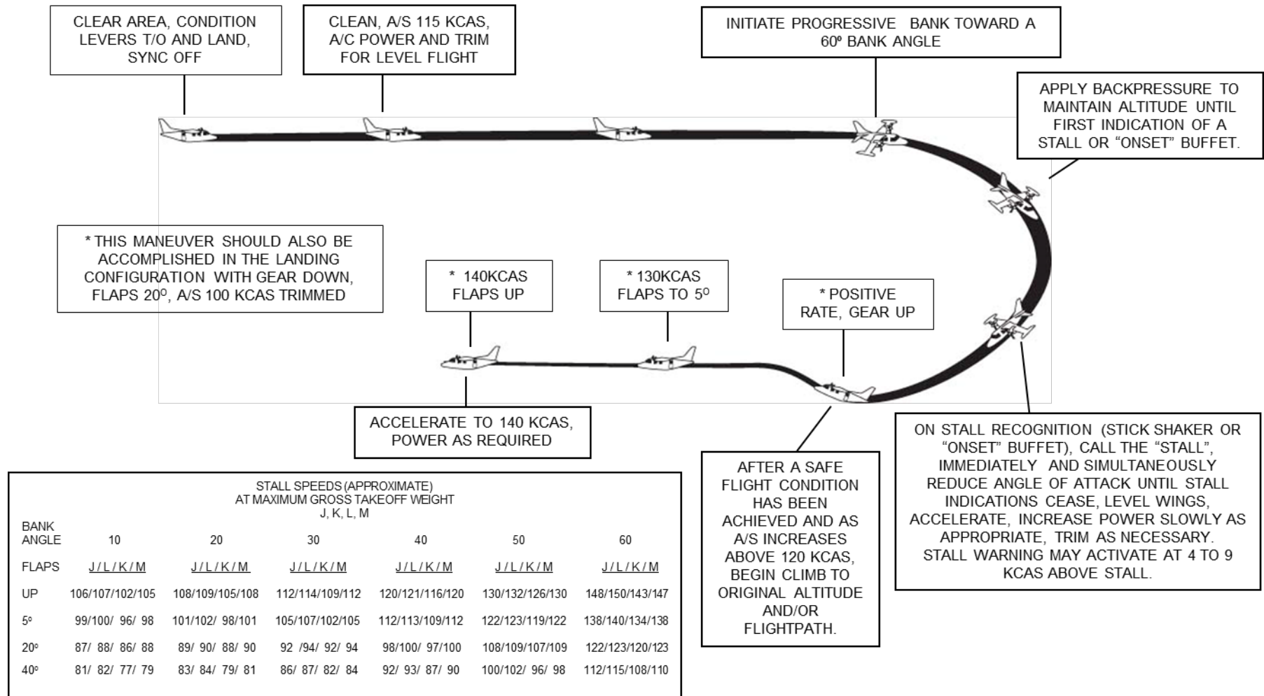
Figure B-11 MU-2B J (-35), K (-25), L (-36), M(-26) ACCELERATED STALLS
