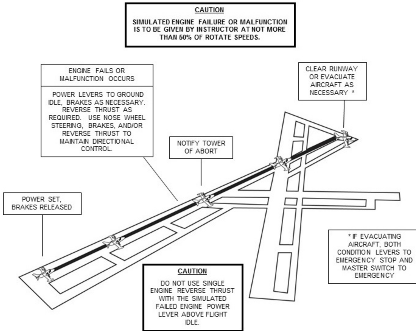
Figure C-3 MU-2B B, D (-10), F (-20), G (-30) TAKE-OFF ENGINE FAILURE ON RUNWAY
