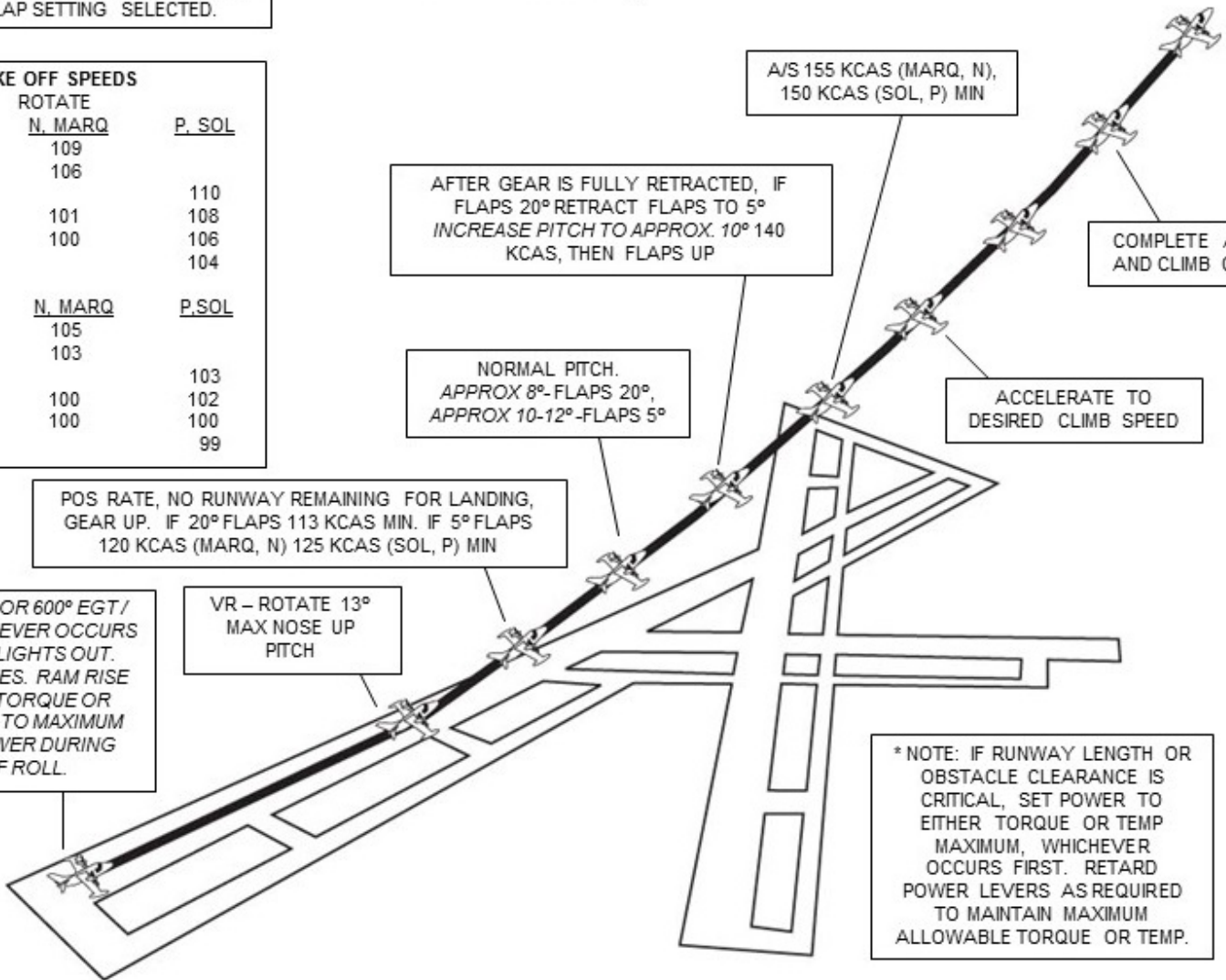
Figure A-1 MU-2B MARQUISE (-60), SOLITAIRE (-40), N (-36A), P (-26A) NORMAL TAKE-OFF, 5° OR 20° FLAPS
