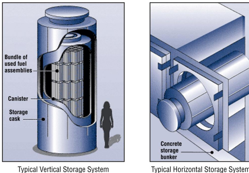
29 Typical Vertical Storage System 30 Typical Horizontal Storage System Figure 3.11-1 Typical Dry Cask Storage Systems. Source: NRC 2020k.
