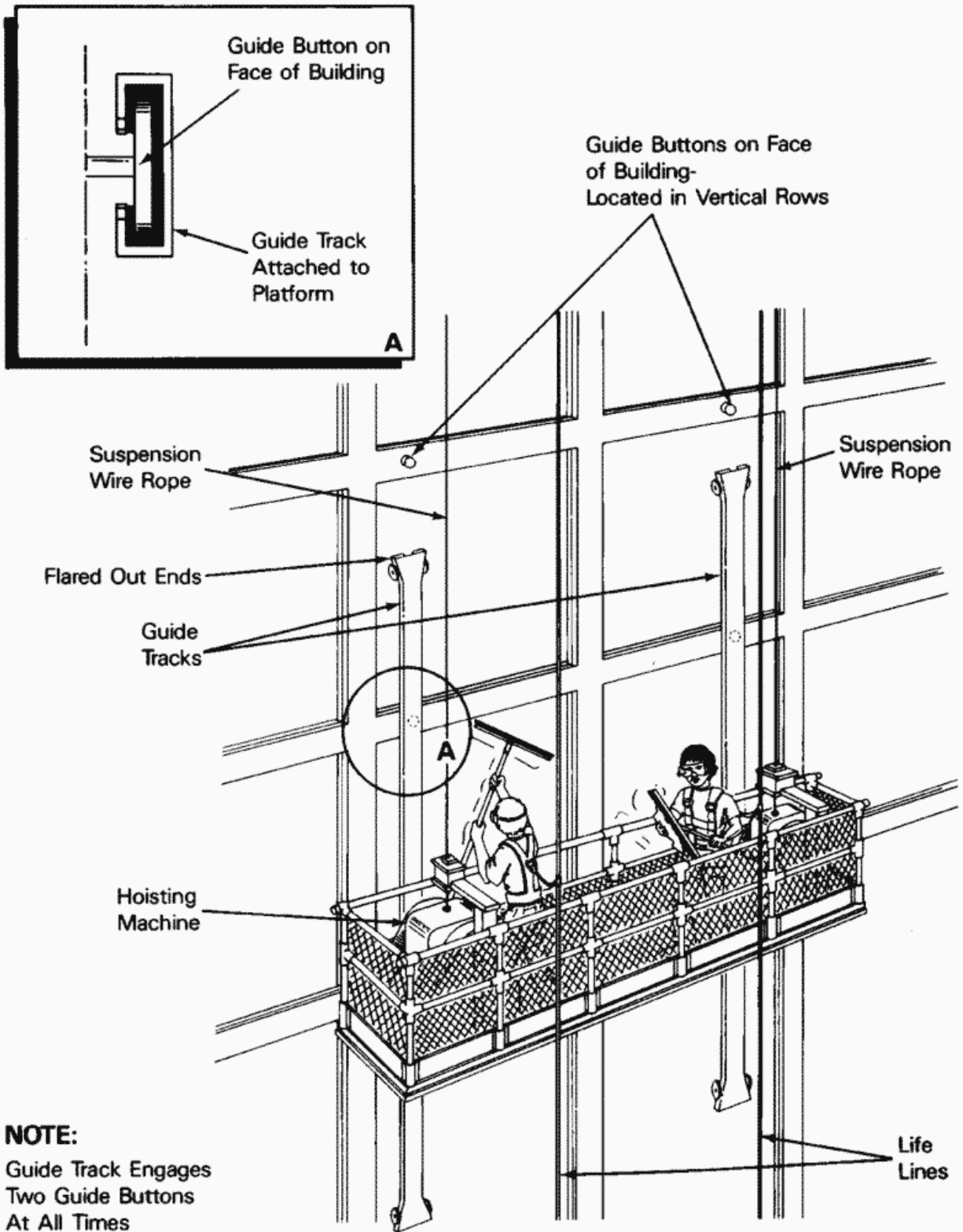
Figure 3. Typical Self-Powered Platform-- Button Guide System
