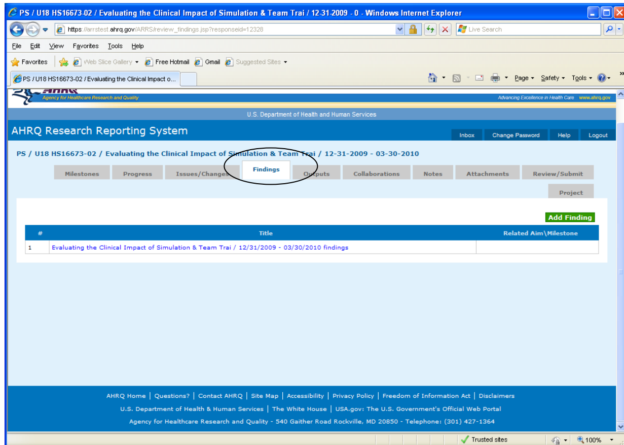
Figure 16: Findings Tab
