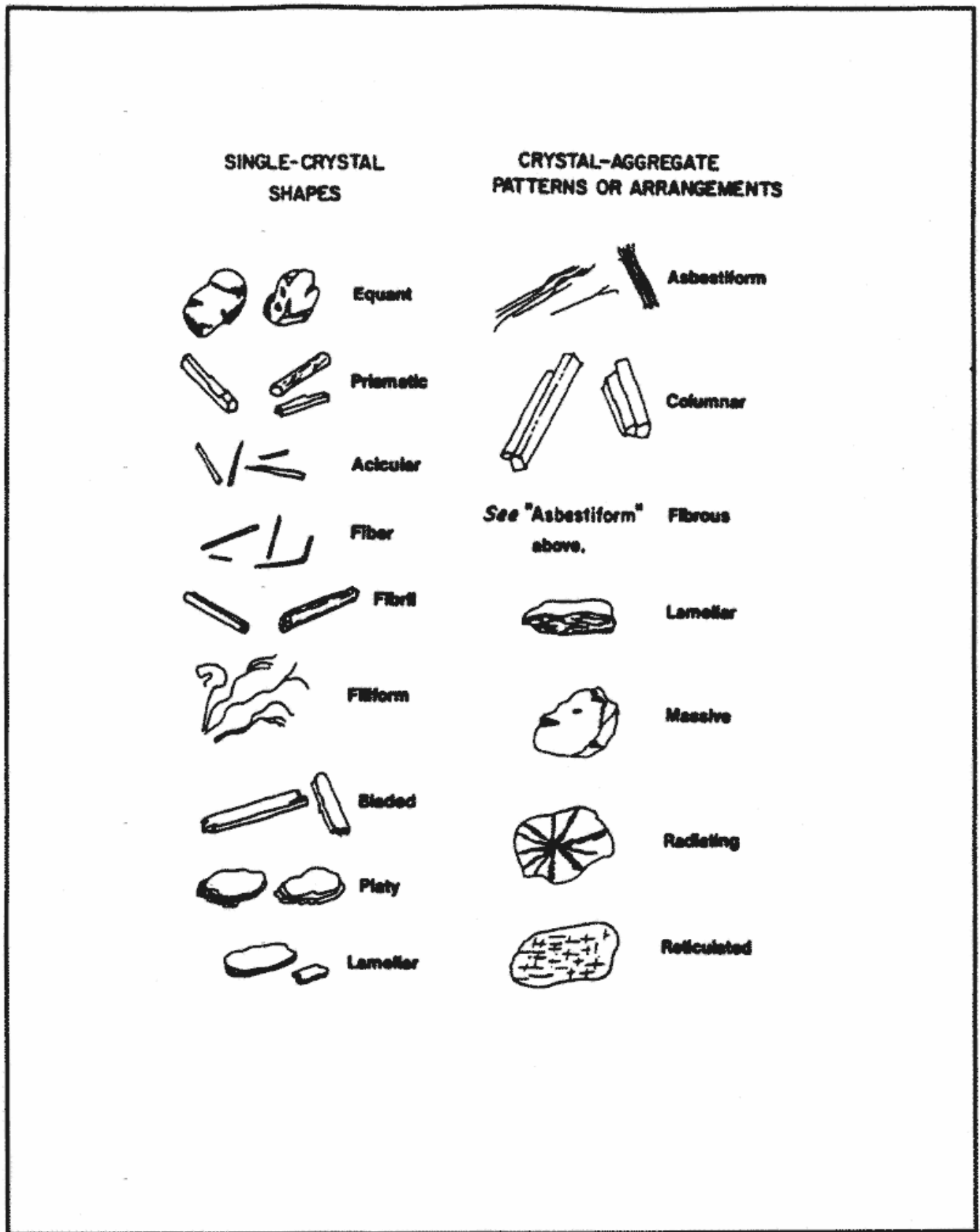
Figure 1. Particle definitions showing mineral growth habits.
