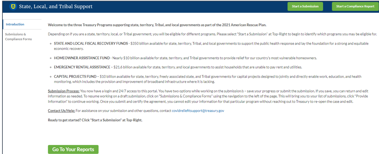
Figure 1 – Landing Page
