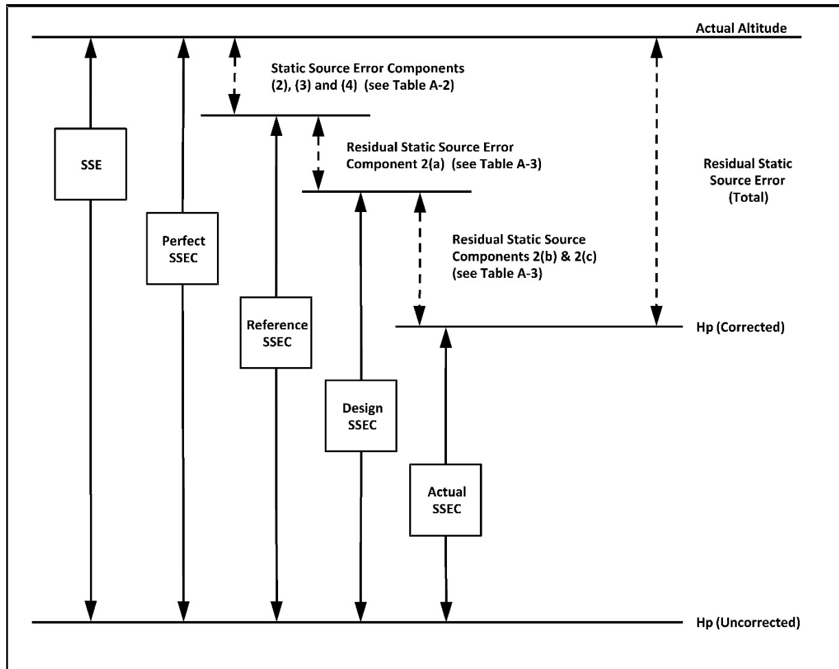
Figure A-4. Static Source Error/Static Source Error Correction Relationships for Altimetry System Error Where Static Line, Pressure Measurement, and Conversion Errors Are Zero
