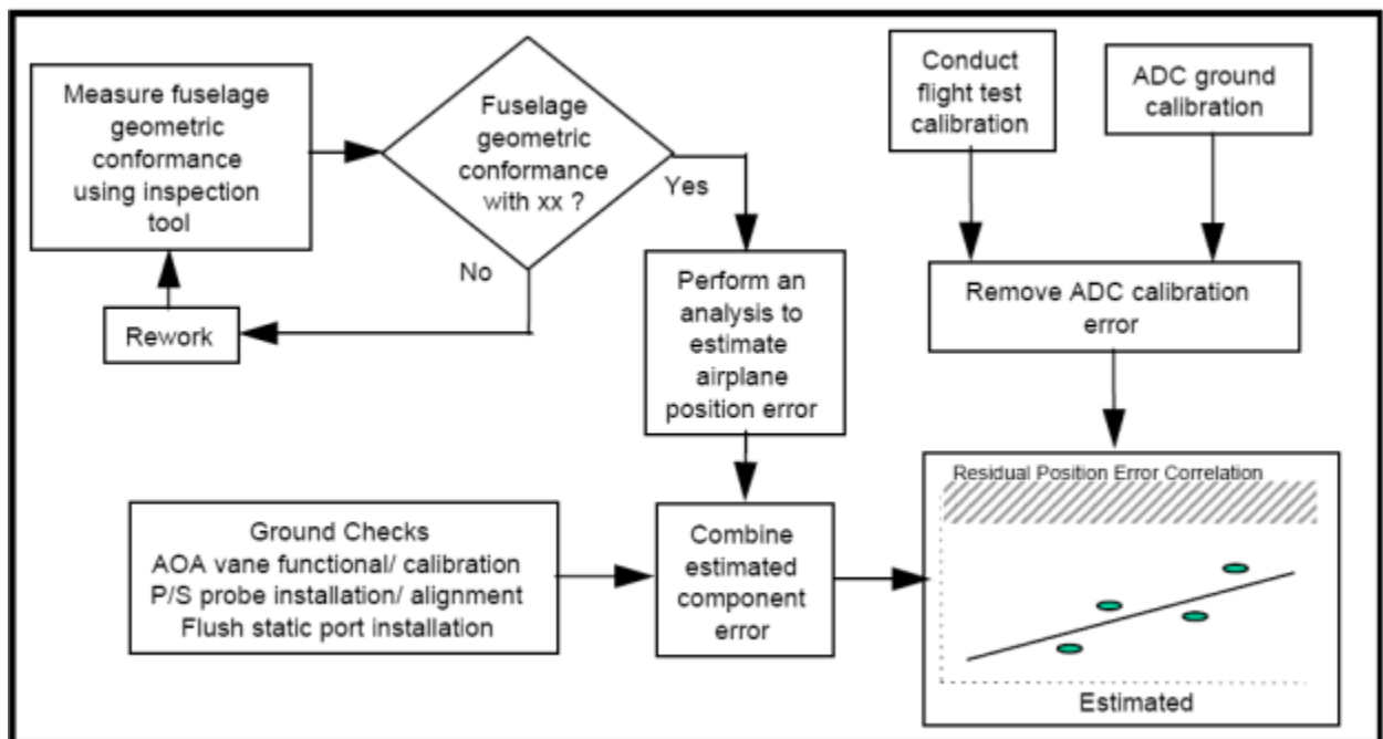
Figure A-6. Compliance Demonstration Ground-To-Flight Test Correlation Process Example
