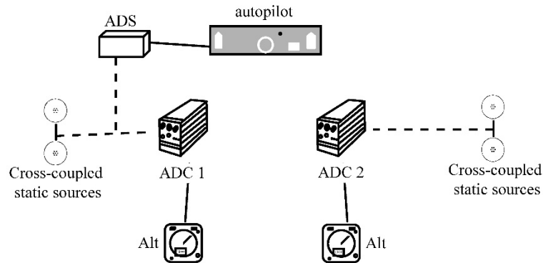
Figure A-1. Example of Air Data System/Autopilot Configuration
