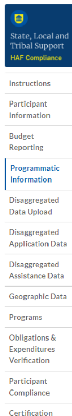
Figure 5 Navigation Bar
