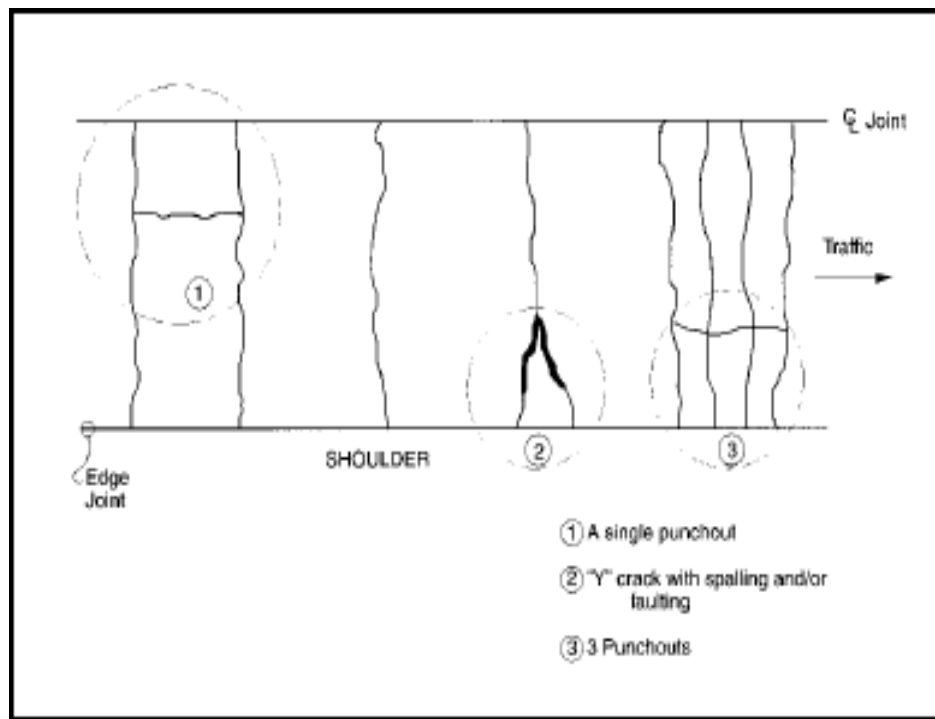
Figure 75: CRCP Fatigue Type Cracking (Punchouts)
