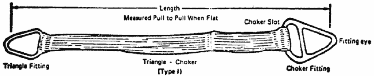
Fig. N-184-6 Basic Synthetic Web Sling Constructions
