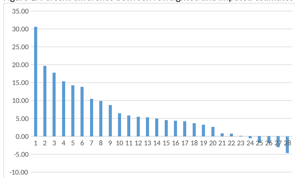
Figure 1. Percent difference between reweighted and imputed estimates for all 28 comparisons.
