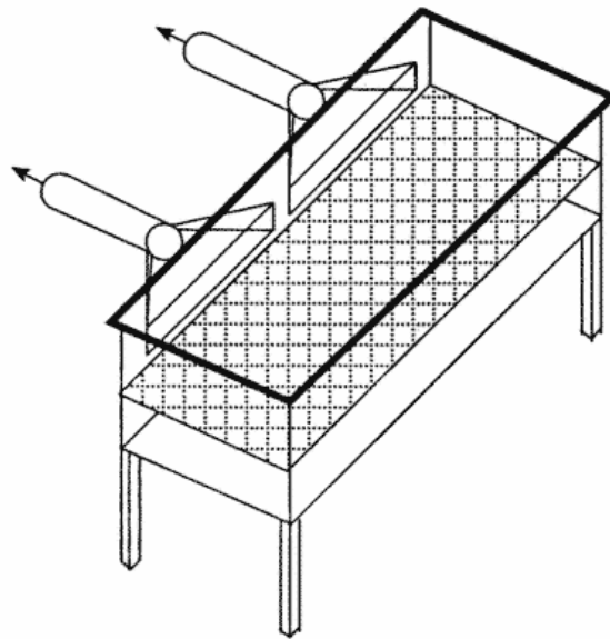
Figure 2 — Downdraft Hood
