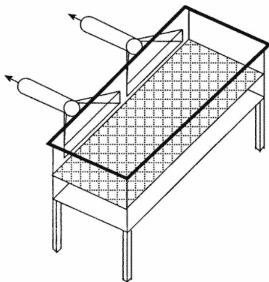
Figure 2 — Downdraft Hood
