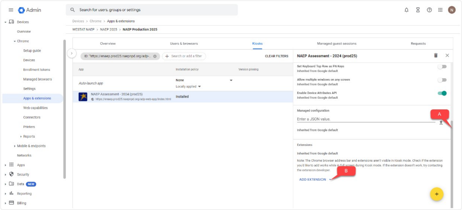
Figure 5. Add Extensions
