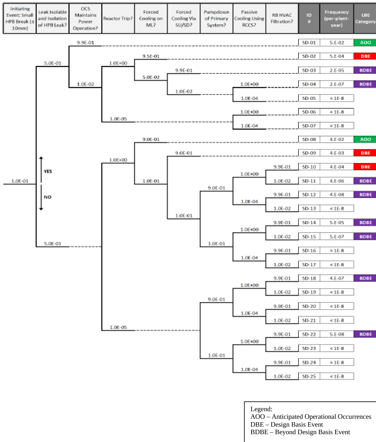
Figure B-2. Helium Depressurization Event Tree (from Ref. B-49)
