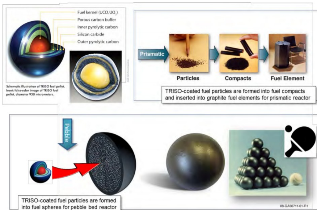
Figure C-2. Depiction of TRISO Fuel Pebbles (from Ref. C- 57 )
