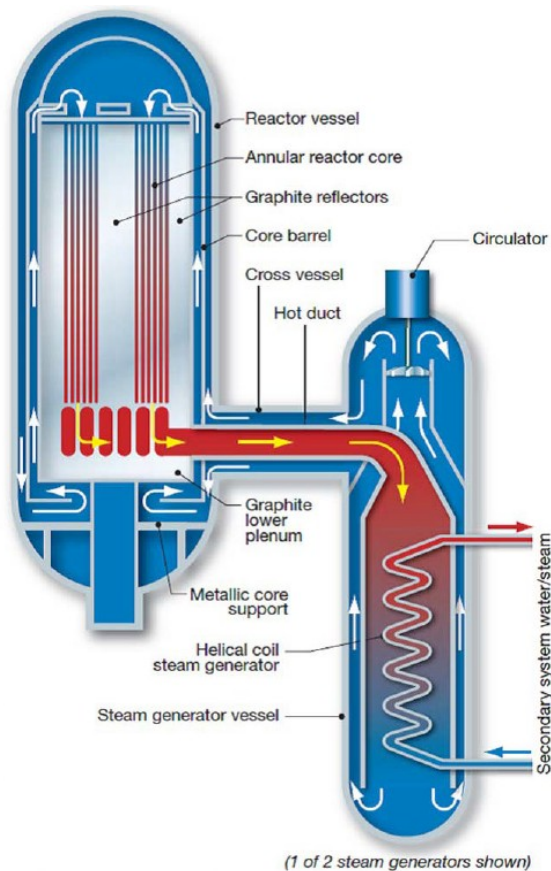
Figure B-1. HTGR Reactor Concept (from Ref. B-48)
