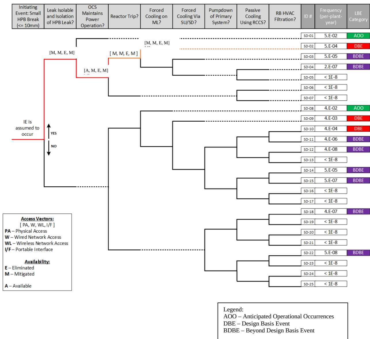
Figure B-8. Analysis for Path Leading to SD-02 (from Ref. B-2)
