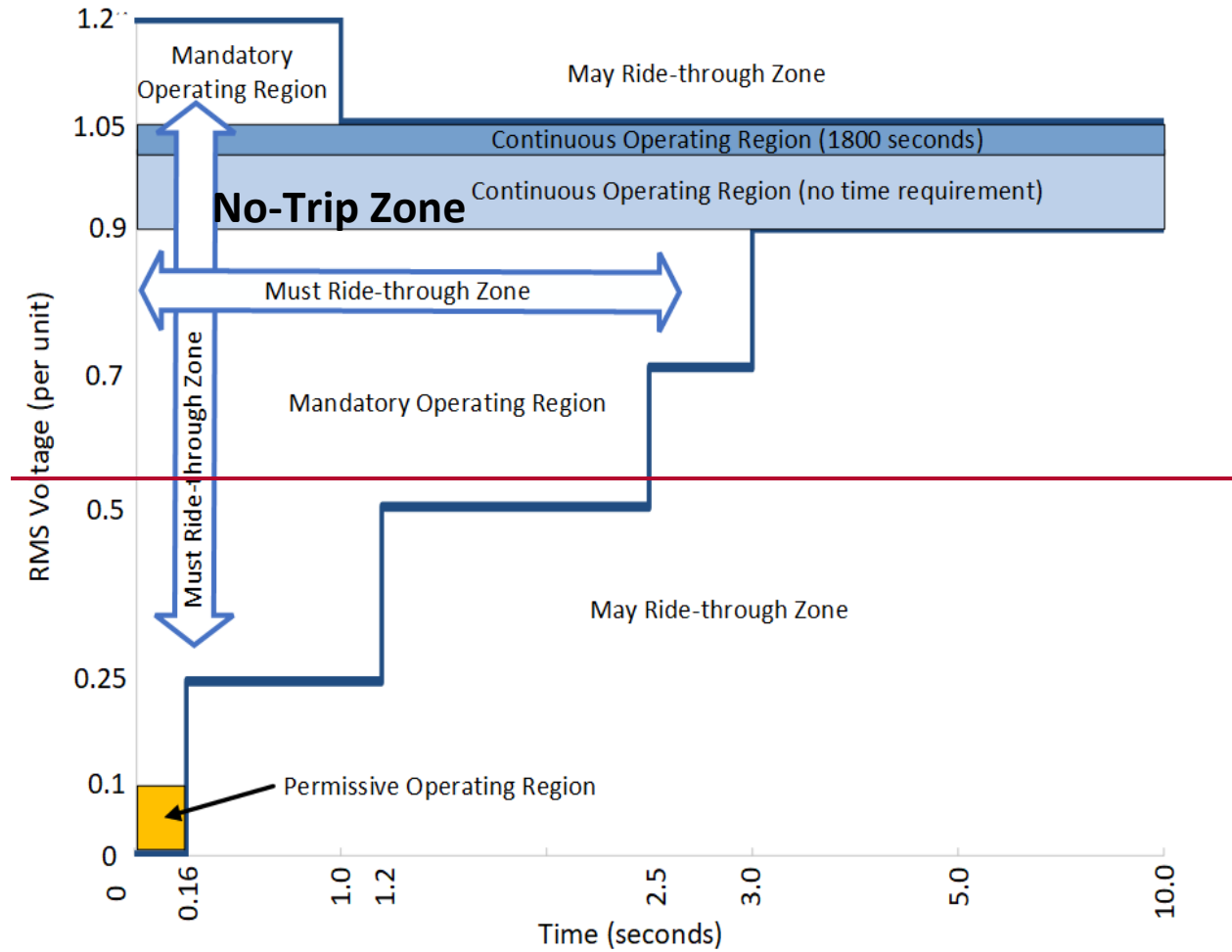
Figure 1: Voltage Ride Through Requirements for AC Connected Wind Facilities
