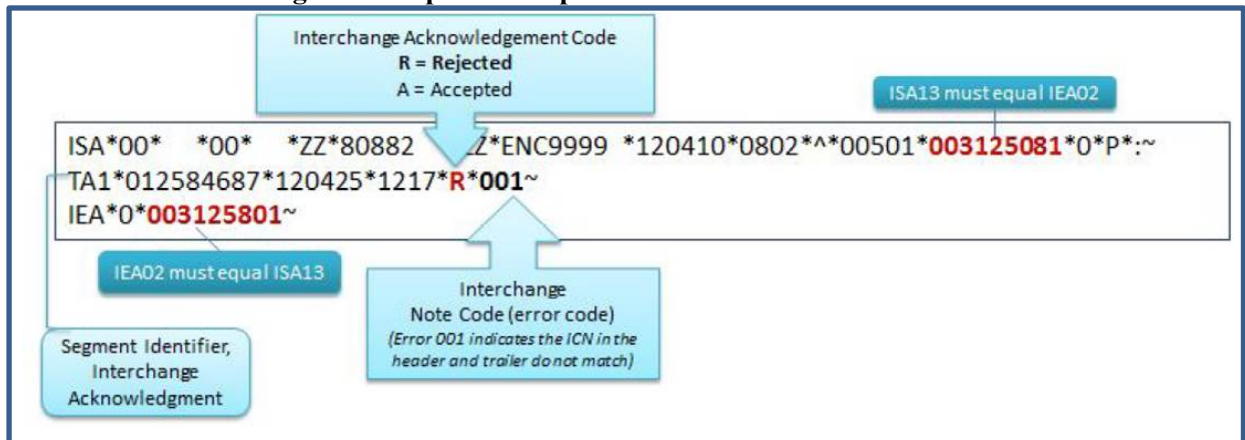
Figure 4.4. TA1 Acknowledgement Report Example
