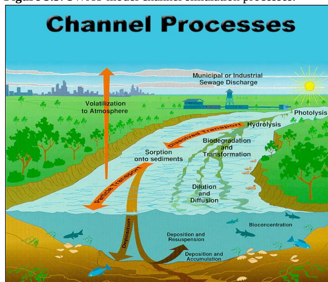
Figure 5.3. SWAT model channel simulation processes.
