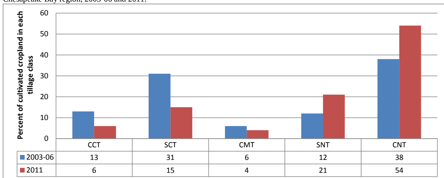
Figure 2.1. Changes in tillage management, as calculated from average annual STIR values for each crop in the rotation in the Chesapeake Bay region, 2003-06 and 2011. 4
