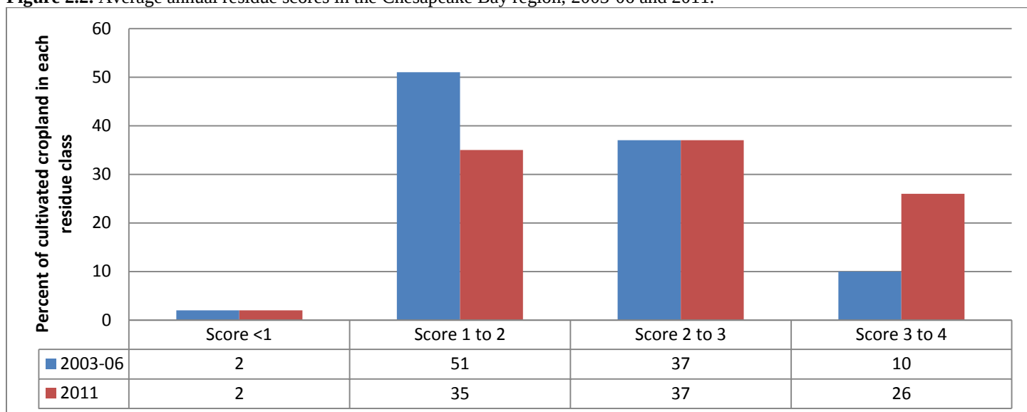
Figure 2.2. Average annual residue scores in the Chesapeake Bay region, 2003-06 and 2011.
