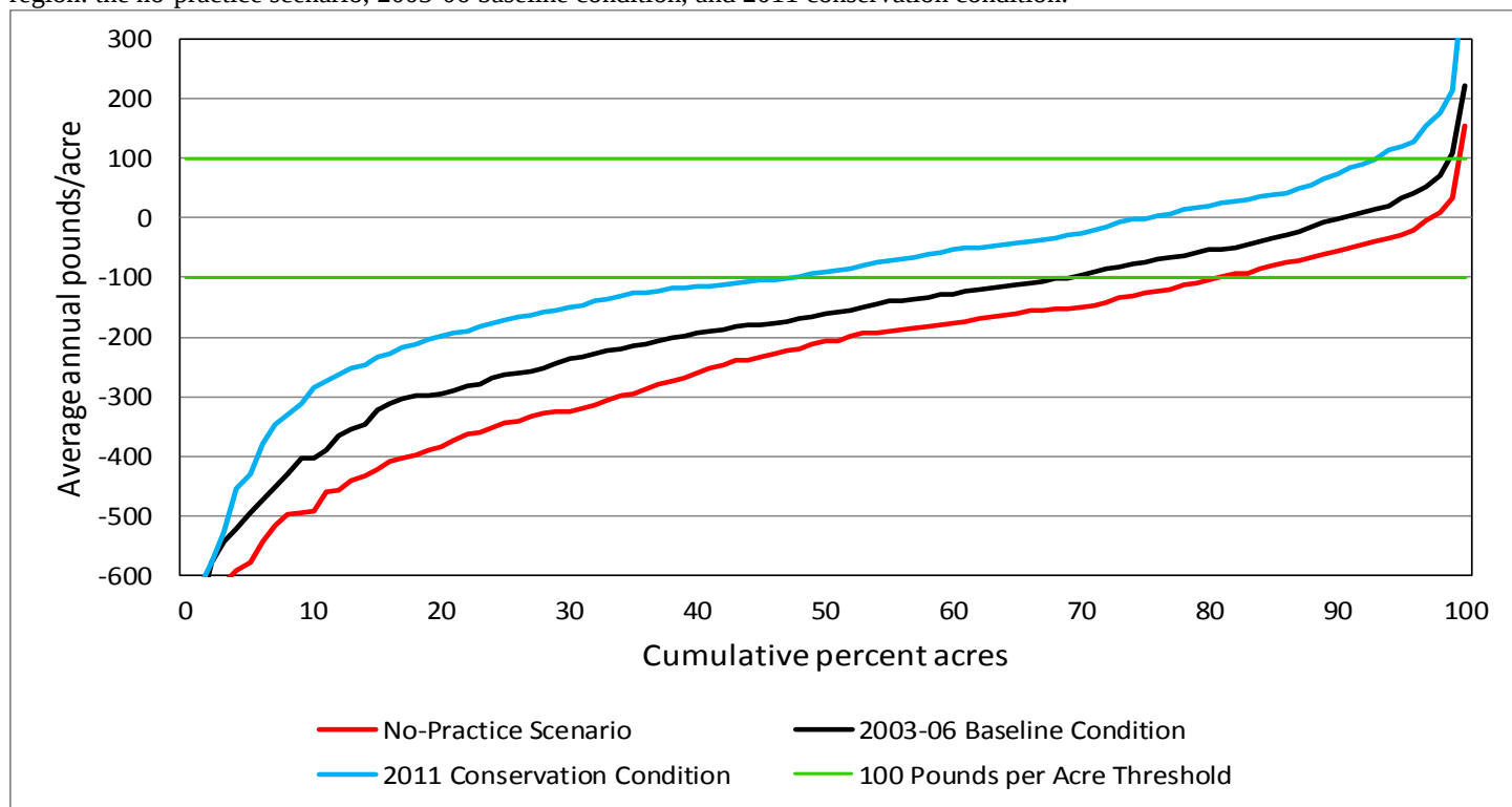
Figure 3.7. Estimates of long-term average annual change in soil organic carbon (SOC) on cropped acres in the Chesapeake Bay region: the no-practice scenario, 2003-06 baseline condition, and 2011 conservation condition.
