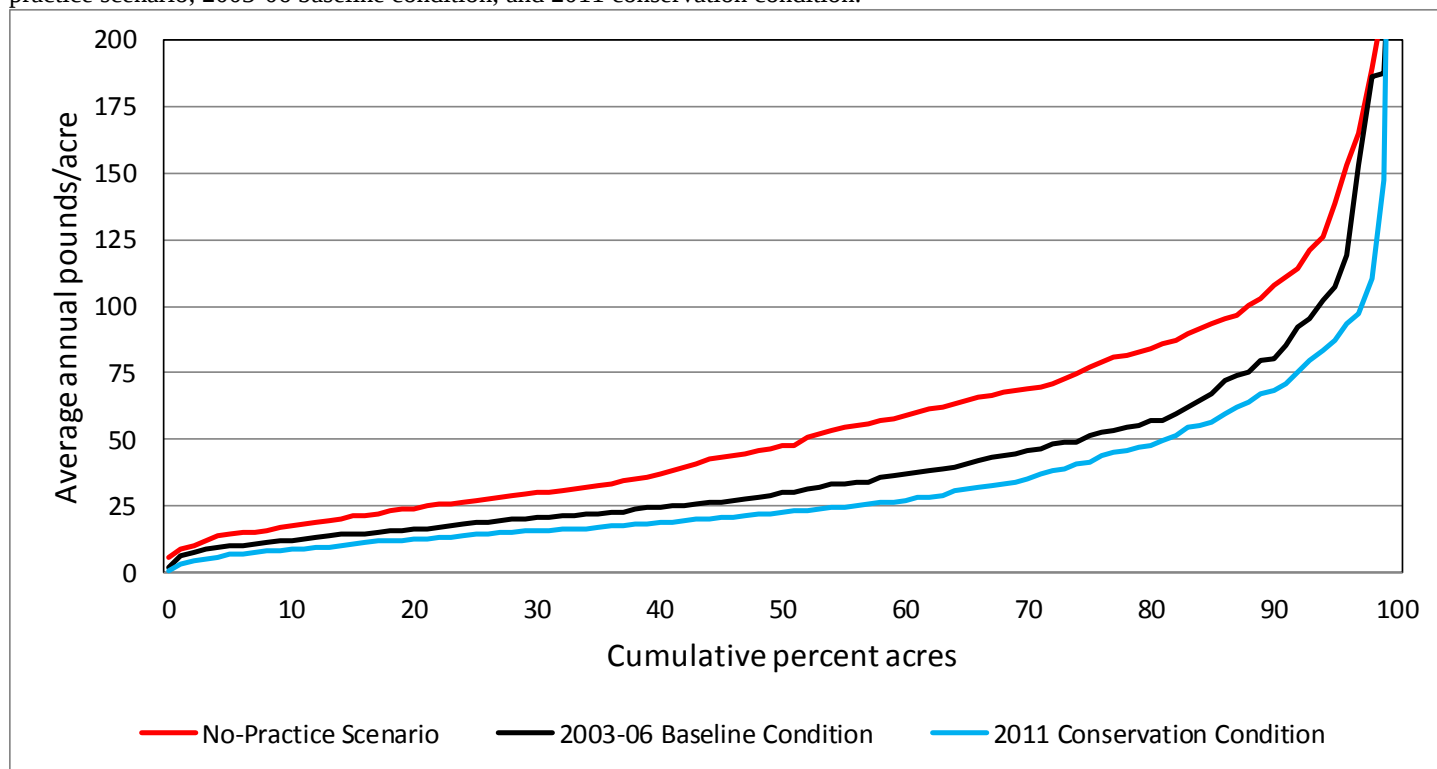
Figure 3.8. Estimates of long-term average annual total nitrogen losses on cropped acres in the Chesapeake Bay region: the no-practice scenario, 2003-06 baseline condition, and 2011 conservation condition.
