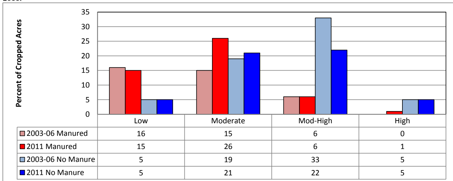
Figure 2.4. Conservation treatment levels for nitrogen application management level in the Chesapeake Bay region, 2003-06 and 2011.
