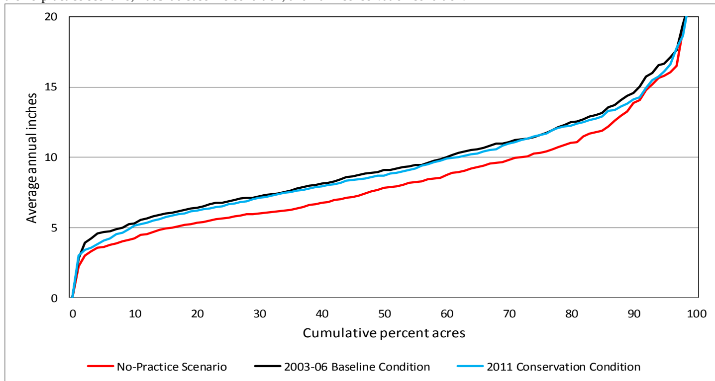
Figure 3.3. Estimates of long-term average annual subsurface flow losses of water on cropped acres in the Chesapeake Bay region: the no-practice scenario, 2003-06 baseline condition, and 2011 conservation condition.
