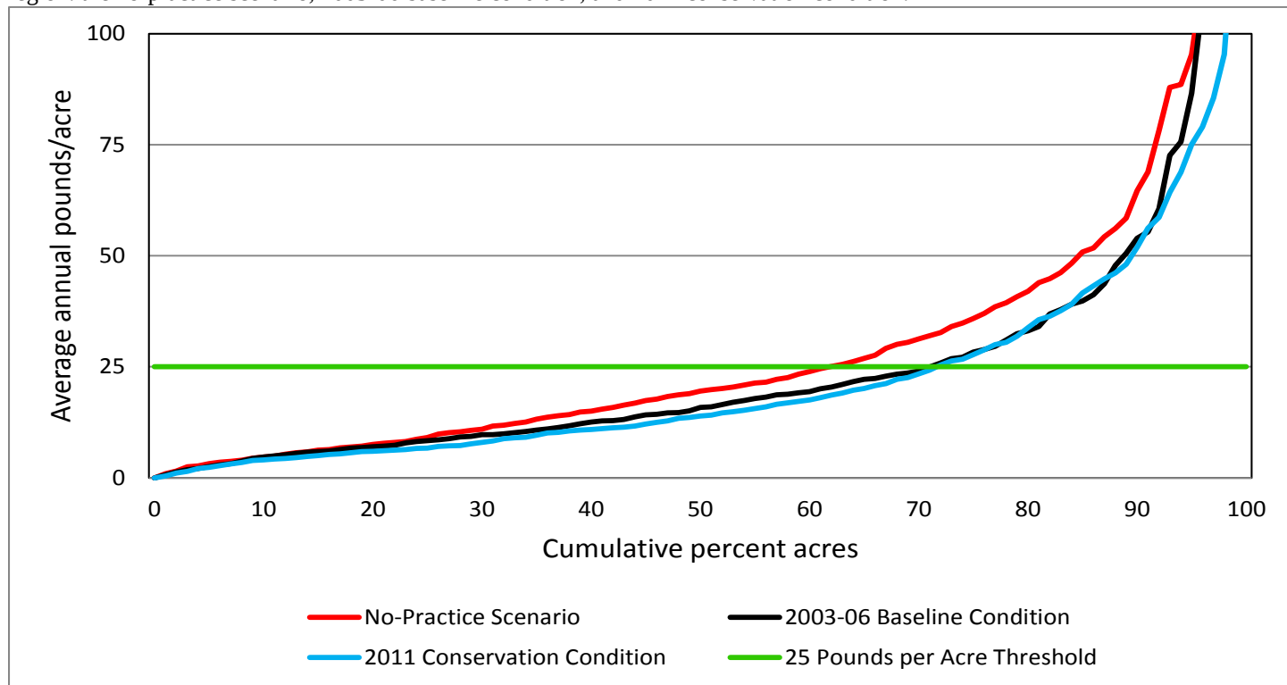
Figure 3.10. Estimates of long-term average annual nitrogen losses in subsurface flow on cropped acres in the Chesapeake Bay region: the no-practice scenario, 2003-06 baseline condition, and 2011 conservation condition.
