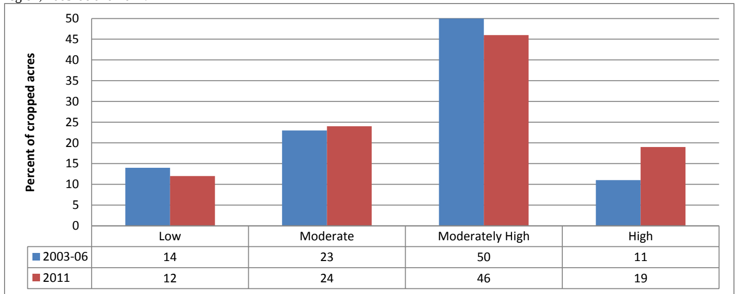
Figure 4.3. Percent of cropped acres in each conservation treatment level for nitrogen leaching control in the Chesapeake Bay region, 2003-06 and 2011.
