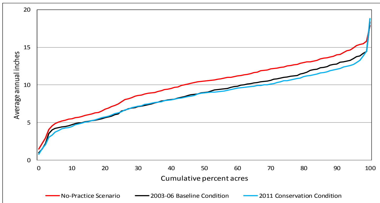
Figure 3.2. Estimates of long-term average annual surface runoff losses of water on cropped acres in the Chesapeake Bay region: the no-practice scenario, 2003-06 baseline condition, and 2011 conservation condition.
