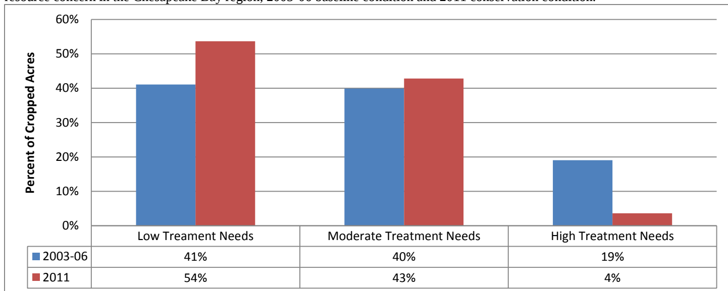
Figure 4.7. Percent of cropped acres with a high, moderate, or low level of need for additional conservation treatment for one or more resource concern in the Chesapeake Bay region, 2003-06 baseline condition and 2011 conservation condition.
