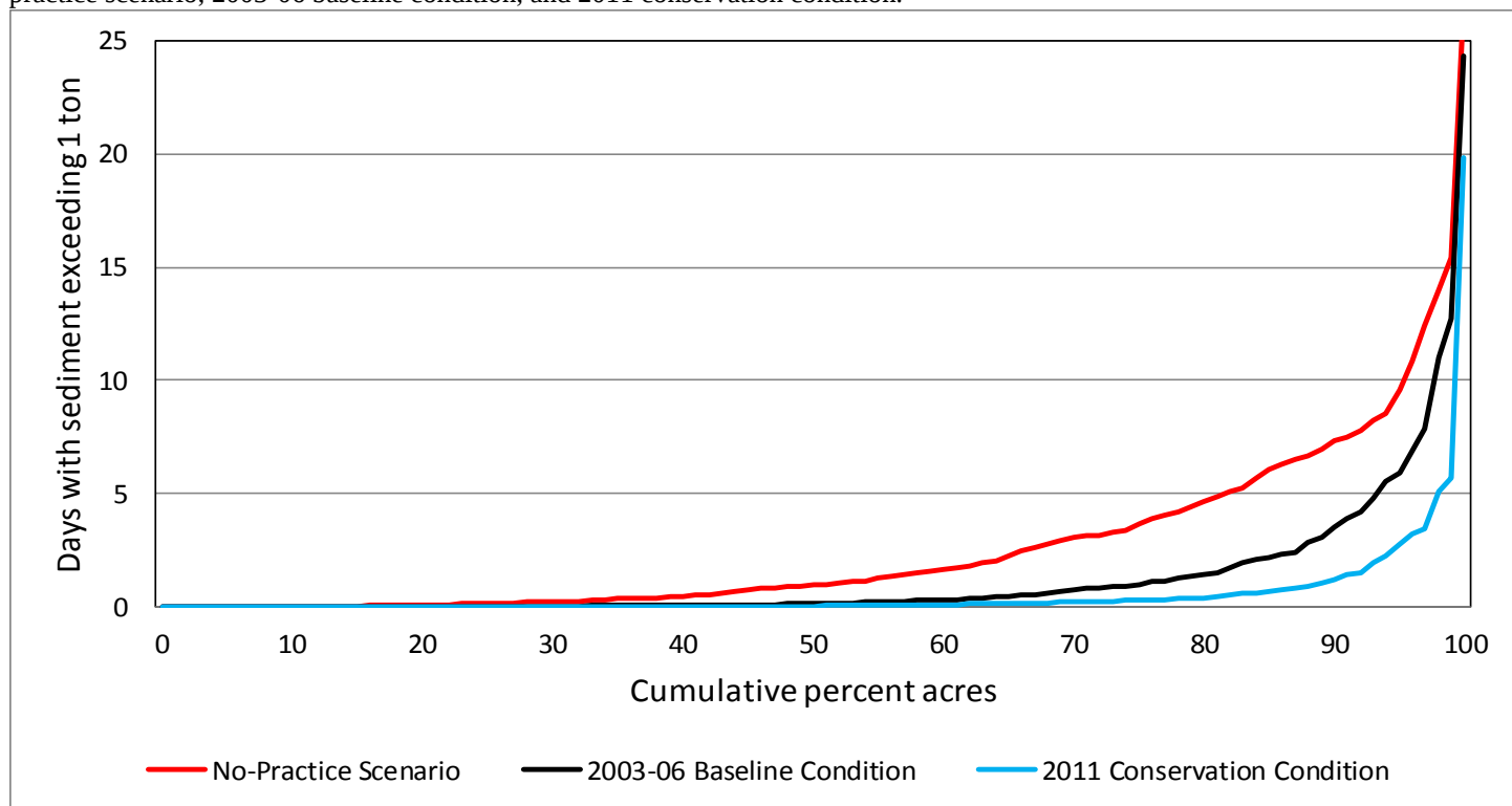
Figure 3.6. Estimates of average number of days each year in which a storm event produced more than 1 ton of sediment loss: the no-practice scenario, 2003-06 baseline condition, and 2011 conservation condition.
