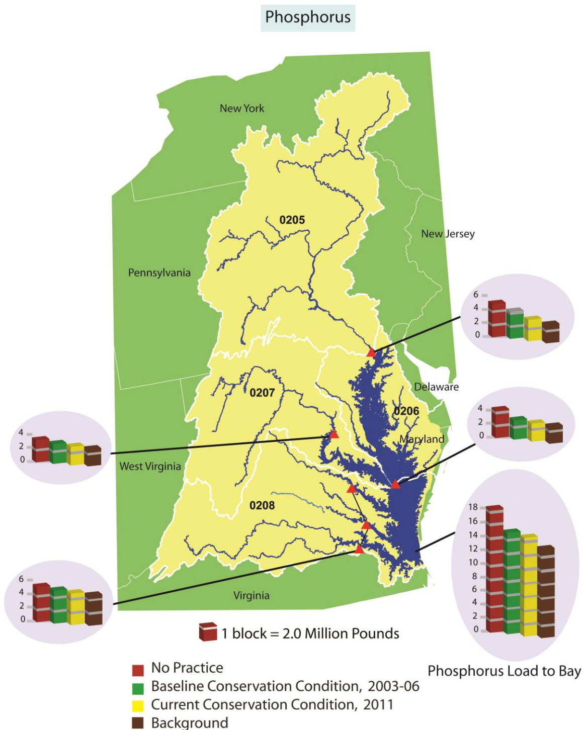
Figure 5.8. Estimates of average annual instream phosphorus loads for the 2003-06 baseline condition and 2011 conservation condition with comparison to the no-practice and background scenarios for subregions in the Chesapeake Bay watershed.*
