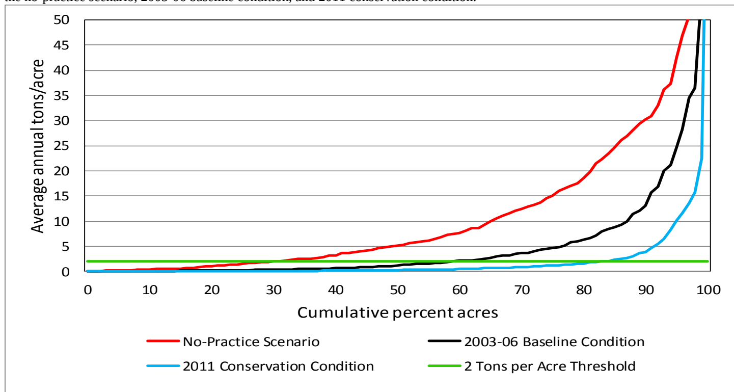
Figure 3.5. Estimates of long-term average annual sediment losses to water erosion on cropped acres in the Chesapeake Bay region: the no-practice scenario, 2003-06 baseline condition, and 2011 conservation condition.
