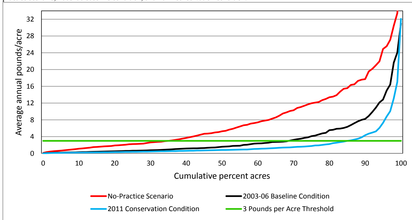
Figure 3.11. Estimates of long-term average annual total phosphorus losses on cropped acres in the Chesapeake Bay region: the no-practice scenario, 2003-06 baseline condition, and 2011 conservation condition.
