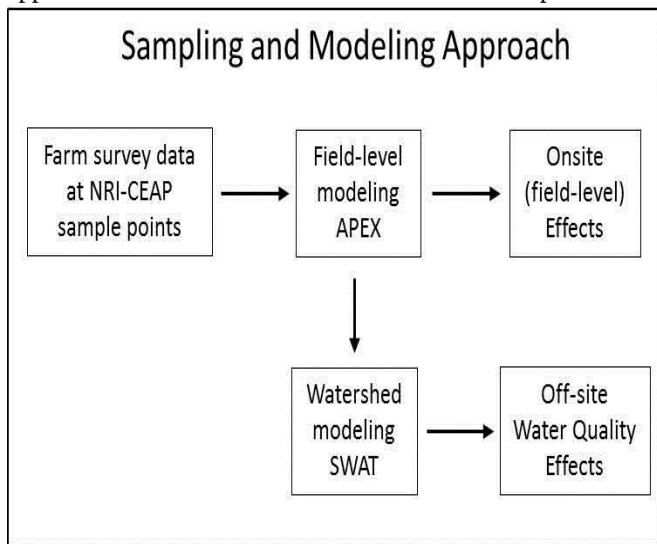
Figure 1.1. Flow diagram of statistical sampling and modeling approach used to simulate effects of conservation practices.
