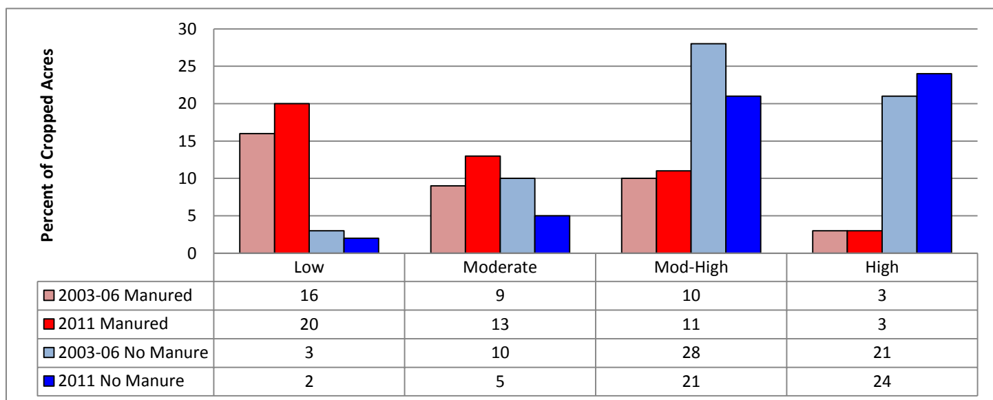
Figure 2.5. Conservation treatment levels for phosphorus application management level in the Chesapeake Bay region, 2003-06 and 2011.
