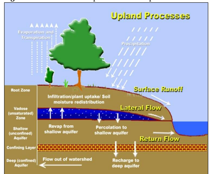
Figure 5.2. SWAT model upland simulation processes.
