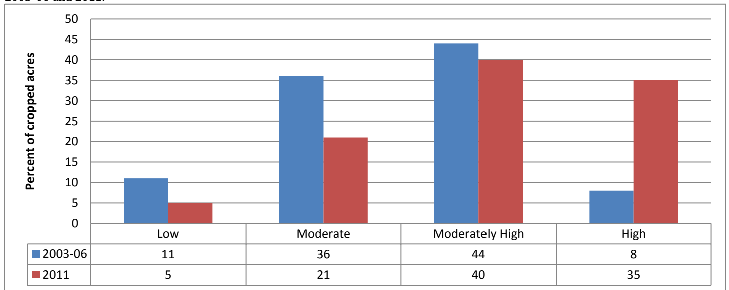
Figure 4.2. Percent of cropped acres in each conservation treatment level for nitrogen runoff control in the Chesapeake Bay region, 2003-06 and 2011.
