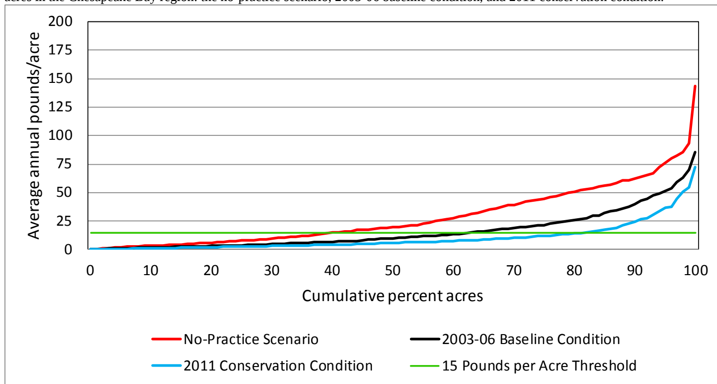
Figure 3.9 Estimates of long-term average annual nitrogen losses with surface runoff (including waterborne sediment) on cropped acres in the Chesapeake Bay region: the no-practice scenario, 2003-06 baseline condition, and 2011 conservation condition.
