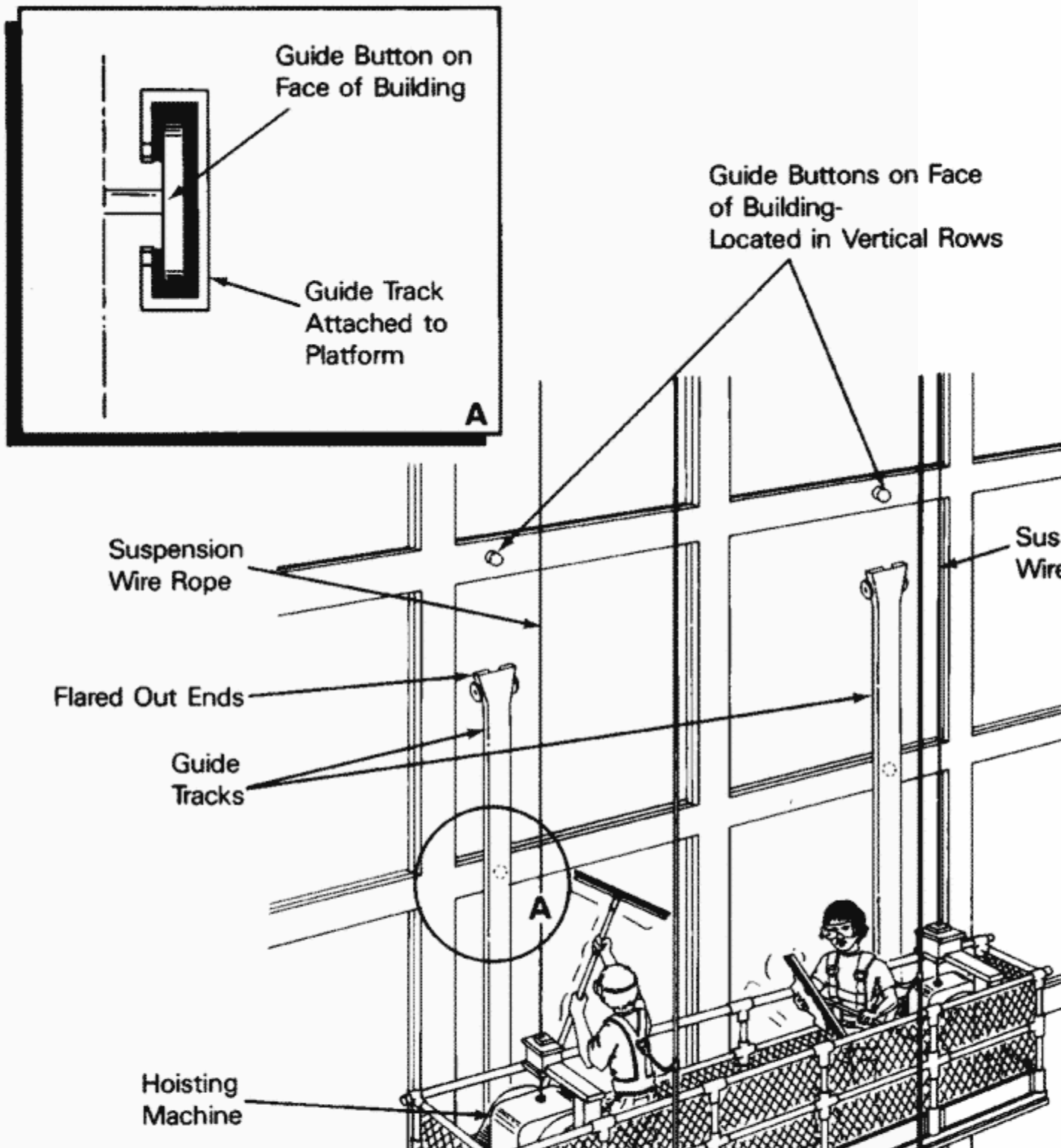
Figure 3. Typical Self-Powered Platform-- Button Guide System
